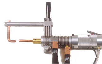
Pneumatic "G" clamp 13.PS.10.86
